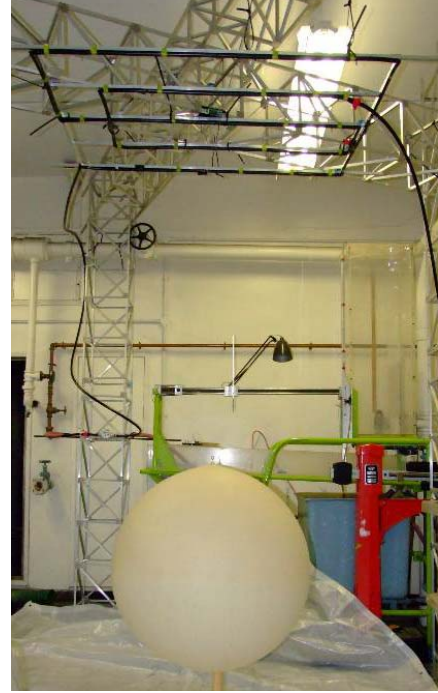
Fig. 5. Drizzle experiment set-up by Nevzat Atakan, see acknowledgements.
