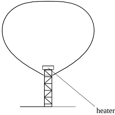
Fig. 2. Electrically heated balloon “Configuration 2”.
