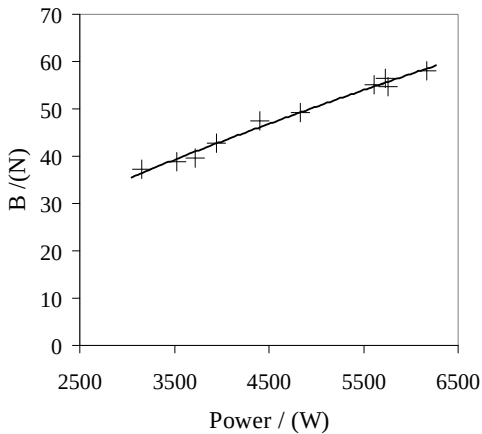
Fig. 3. Buoyant lift vs. electrical power input, for “Configuration 2”.
