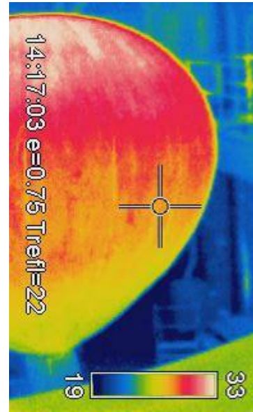
Fig. 4. Infra-red image of heated envelope (“Configuration 2”), showing increase in wall temperature towards the crown.
