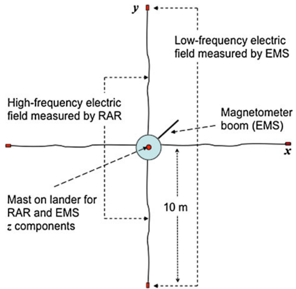
Fig. 16 The radio astronomy receiver (RAR) and electromagnetic sounding (EMS) experiment utilize the same antennas to measure all three components of the high- and low- frequency electric fields, respectively. RAR measures differences in voltage of the separate antennas, whereas EMS measures differences in voltage between the antenna end points
